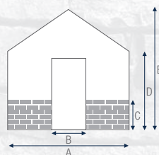
Feature Dwarf Wall 12'x8' (Nominal), Green, Full Sheet Toughened Glass
